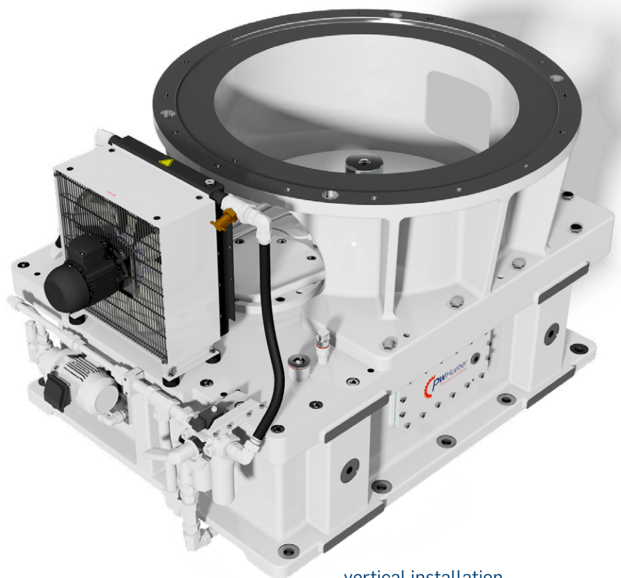
vertical installation
